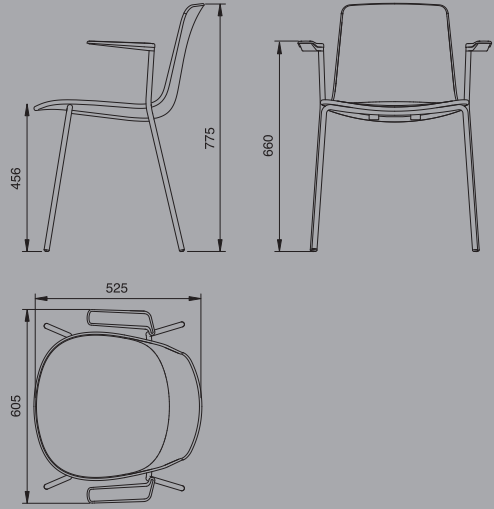
LOTTUS CON BRAZOS ALA WITH WING-SHAPED ARMRESTS
