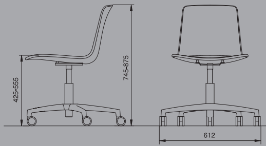
LOTTUS GIRATORIA SIN BRAZOS SWIVEL CHAIR WITHOUT ARMRESTS
