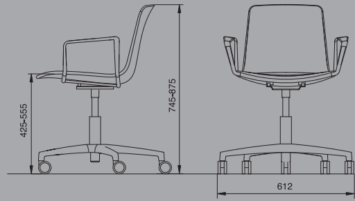
LOTTUS GIRATORIA CON BRAZOS ACERO SWIVEL CHAIR WITH STEEL ARMRESTS
